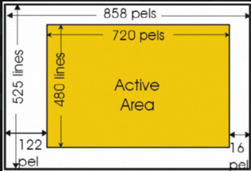
NTSC 525/60 : 60 field/sec
